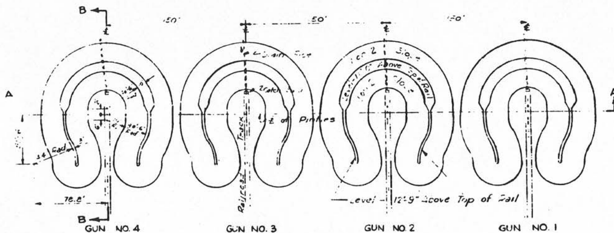
PLAN OF REVETMENTS
